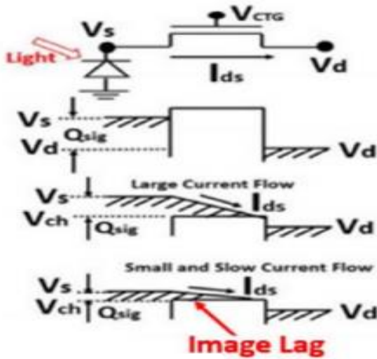
Serious Image Lag of Floating N+P Single Junction Photodiode.
