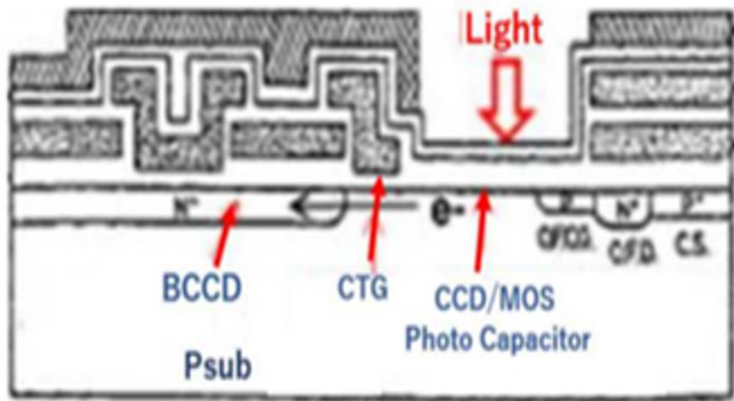
ICX-008 Sony ILT CCD Image Sensor Structure
