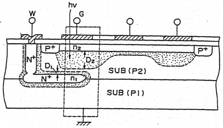
VOD on CCD/MOS Photo Capacitor
