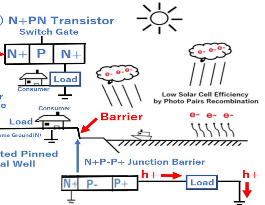
(1) N+P-P+ Single Junction Solar Cell
