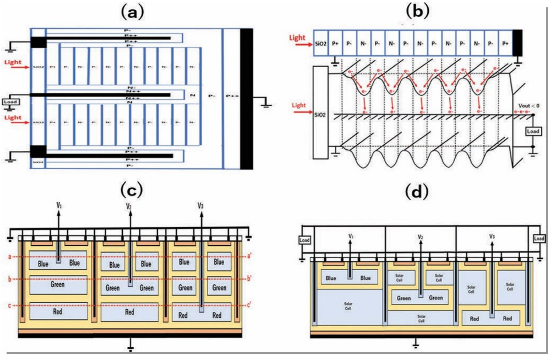
Figure 10. (a) The cross-sectional view and (b) the potential profile of a multi-junction pinned photodiode type solar cell; (c) a color-filter-less color image sensor; (d) a combination of a color-filter-less color image sensor and a solar cell
