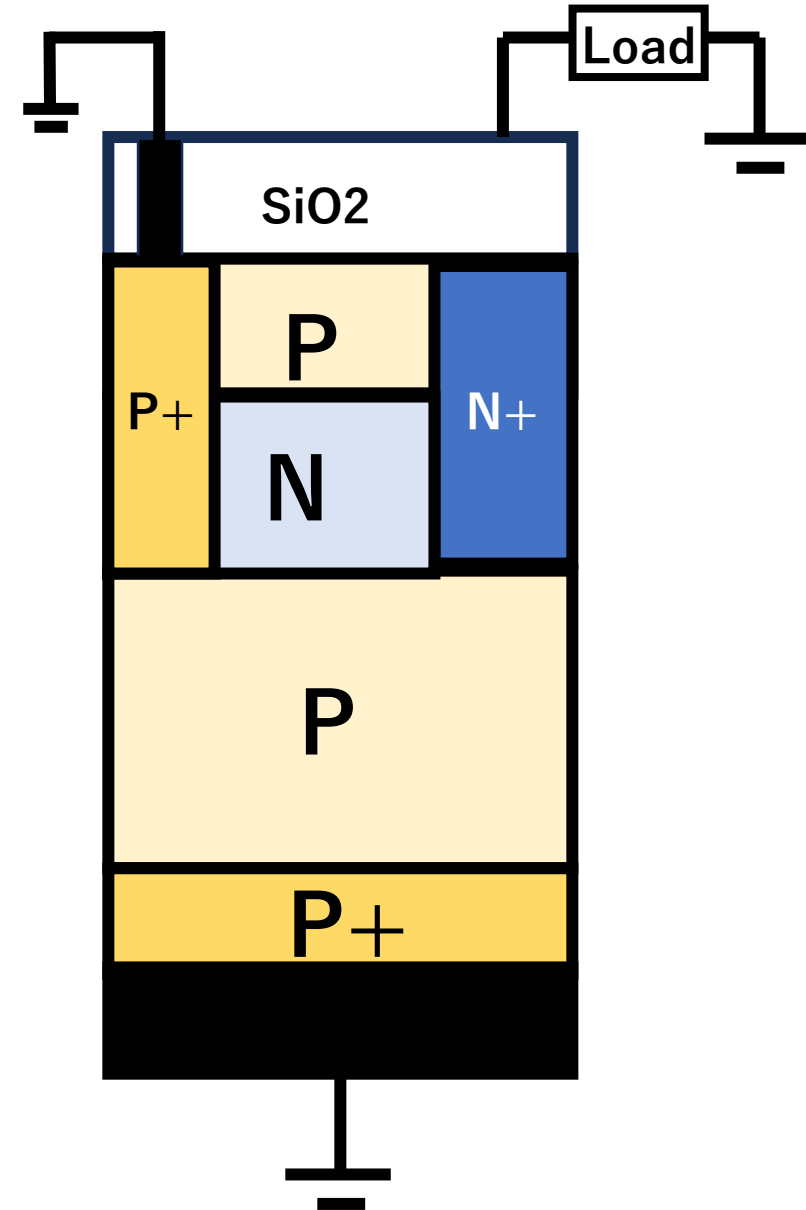
(c) JPA2020-131313 Double Junction Solar Cell
