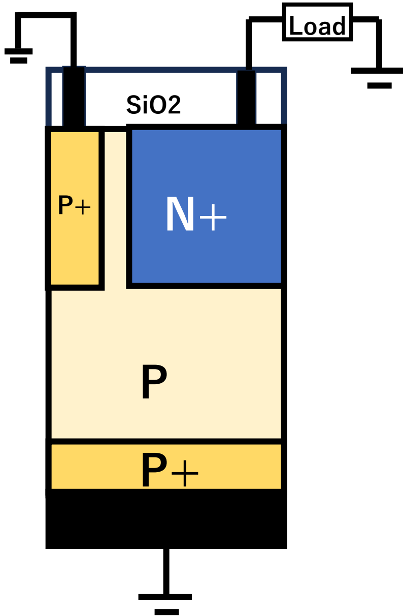
(a) Conventional N+P Single Junction Solar Cell
