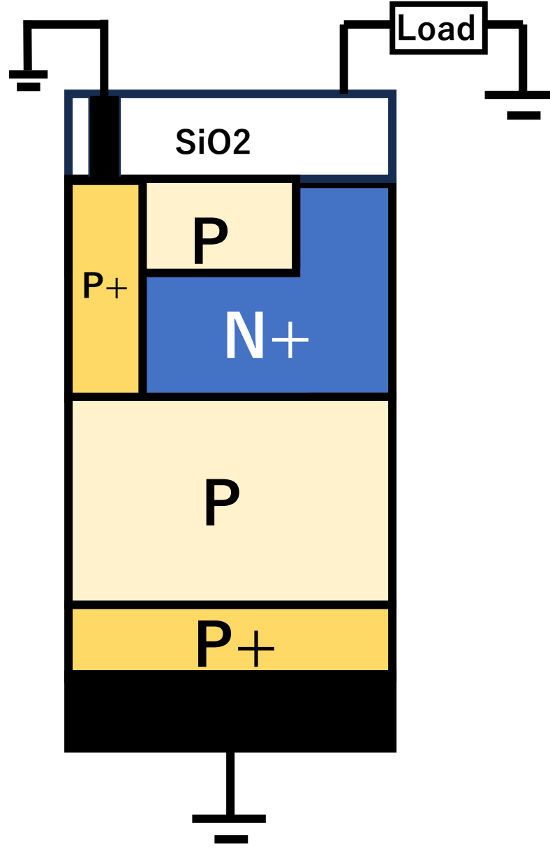
(b) Modified PN+P Double Junction Solar Cell
