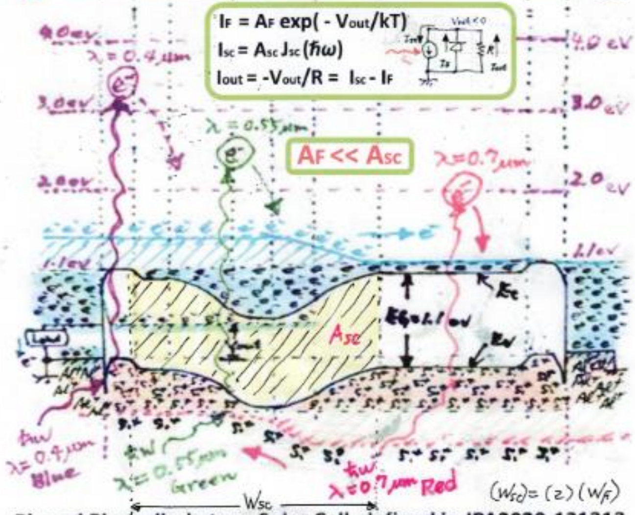
Pinned Photodiode type Solar Cell defined in JPA2020-131313 filed on August 1, 2020 by Yoshiaki Hagiwara
