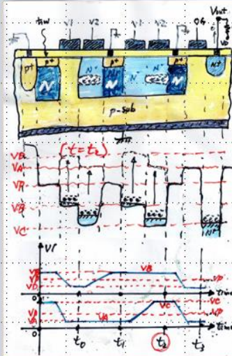
Concept of Virtual Gate applied in two-phase CCD analog delay line
