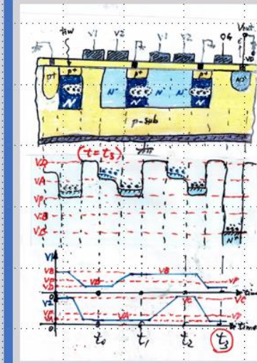
Concept of Virtual Gate applied in two-phase CCD analog delay line
