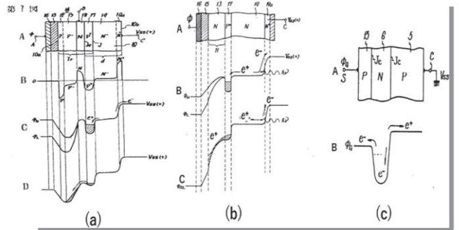
Figure 2: Reproductions from the Japanese Patent Applications of (a) the N+N-P+N-P triple junction PPD, (b) the N+N-P+N double junction PPD, and (c) the PNP double junction PPD.
