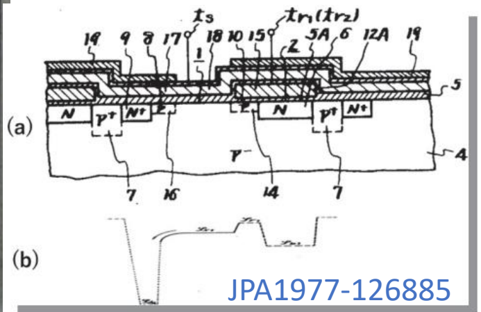
Figure 7: Figures reproduced from Japanese Patent Application JPA1977-126885: (a) sensor, (b) potential profile for the OFD punch-through action.
