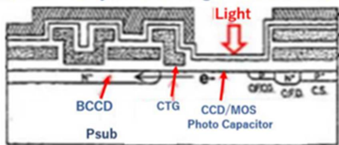
ICX-008 Sony ILT CCD Image Sensor Structure
