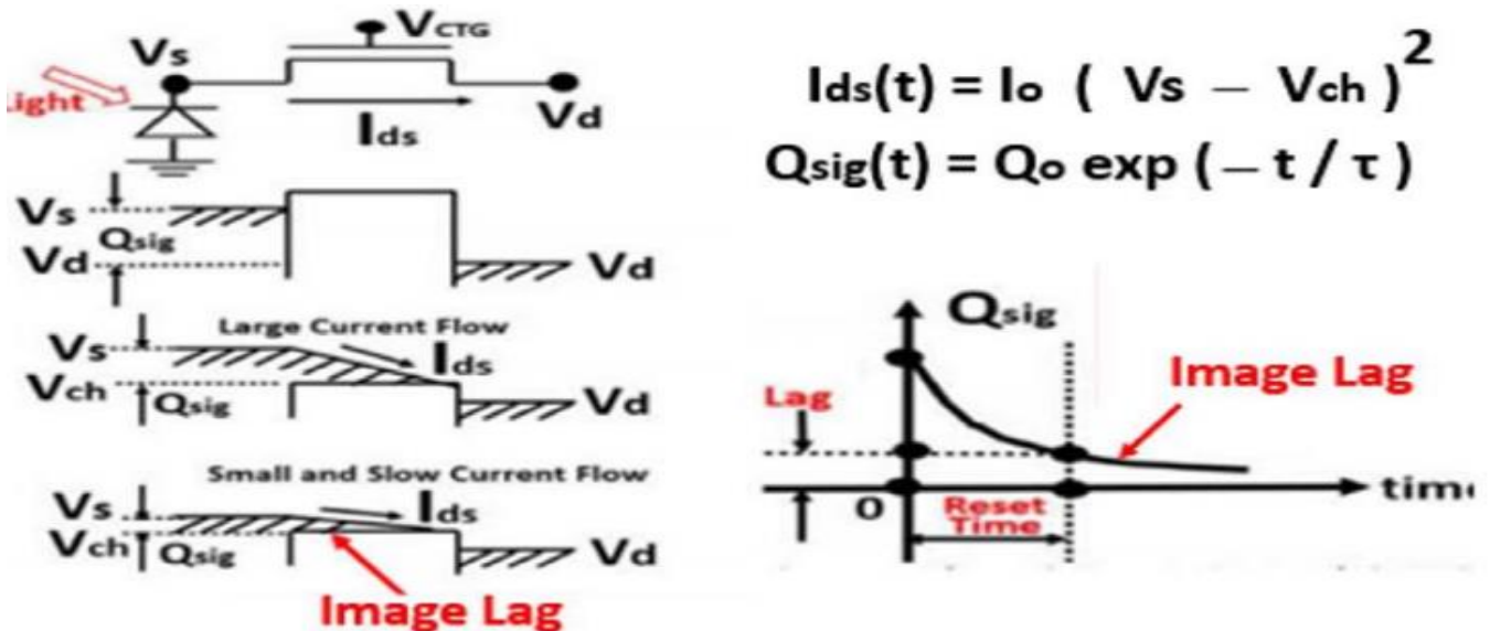
Serious Image Lag of Floating N+P Single Junction Photodiode.
